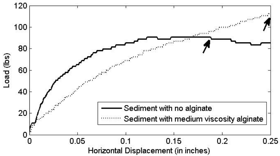
Figure 2: Example of shear curves. Arrows highlight where peak shear values are taken for the different curve shapes encountered.
