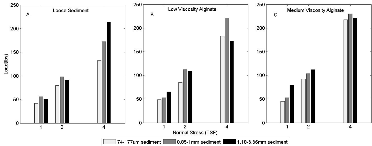
Figure 3: Peak shear of A) Sediment without alginate, B) Sediment gelled with low viscosity alginate and C) Sediment gelled with medium viscosity alginate at different applied normal stresses.
