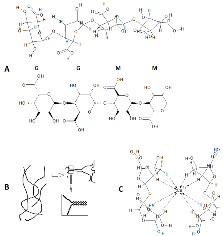
Figure 1: The different residues of Alginate arranged in MM and GG blocks are shown in A; the mechanism for cross linking where cations fit between the chains in the egg-box model shown in B; and the points of interaction between calcium and alginate shown in C.
