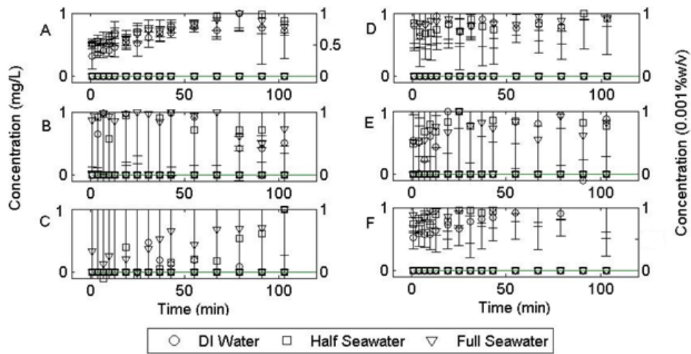
Figure 7: Normalized leaching from Sediment-gels. Low viscosity gel data is on the left while medium viscosity gel data is on the right. Methylene Blue diffusion is graphed with a solid line while naphthalene diffusion is graphed as points only. Sediment size is in decreasing order from the top with 1.18-3.36mm sediment in A and D; 0.850-1mm sediment in B and E; and 74-177 \mu\text{m} in C and F. Solution are buffered to a pH of 5.8 and a temperature of 24°C
