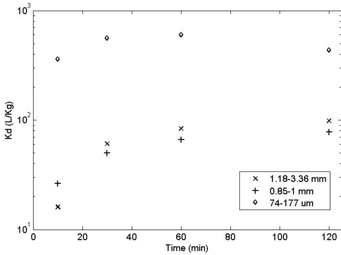
Figure 6: Sorption coefficient over time for Methylene Blue to sediment
