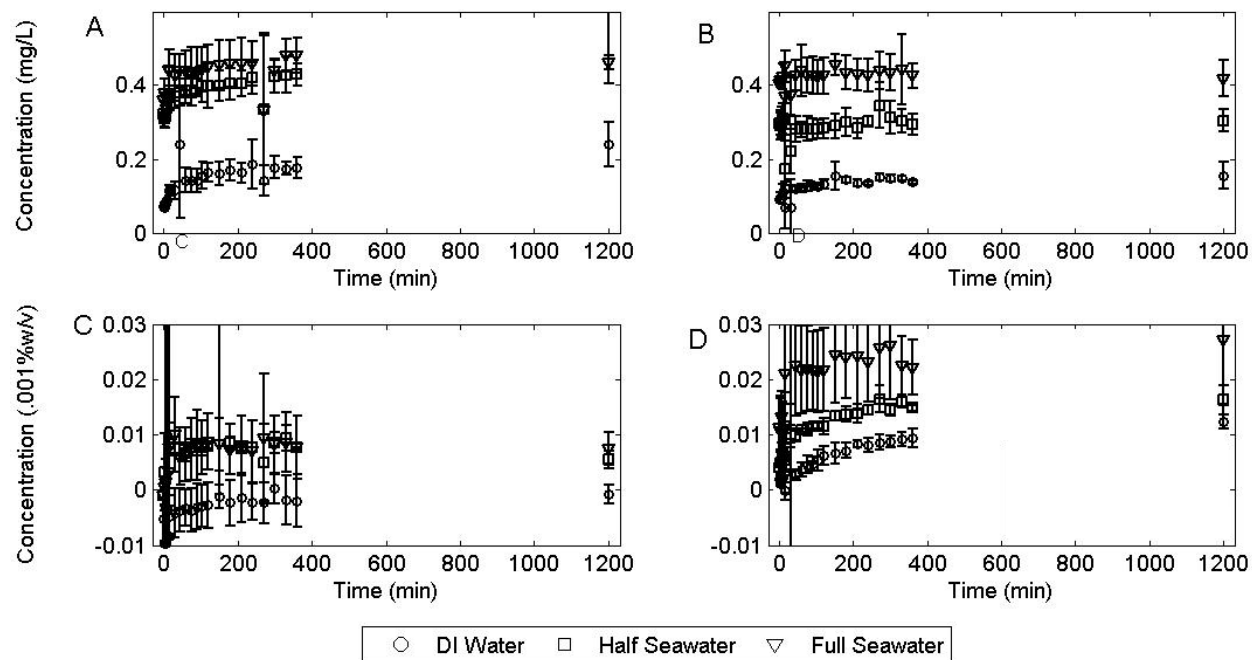
Figure 4: Change in concentration of Naphthalene released from A: low viscosity alginate and B: medium viscosity as well as Methylene Blue released from C: low viscosity alginate and D: medium viscosity alginate into unbuffered solutions of DI water, Half and Full seawater at 24°C
