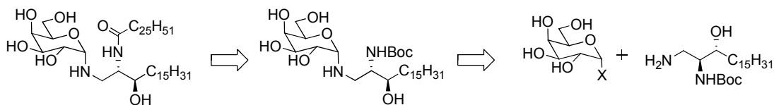
Figure 11: Approach to revised \alpha -N-GalCer
