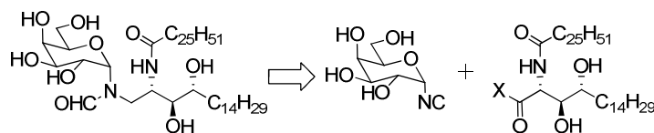
Figure 10: Approach to \alpha - N -formyl- N -GalCer
