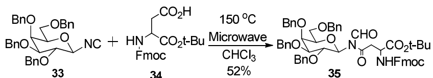
Scheme 10: Danishefsky's reported acyl transfer reaction
