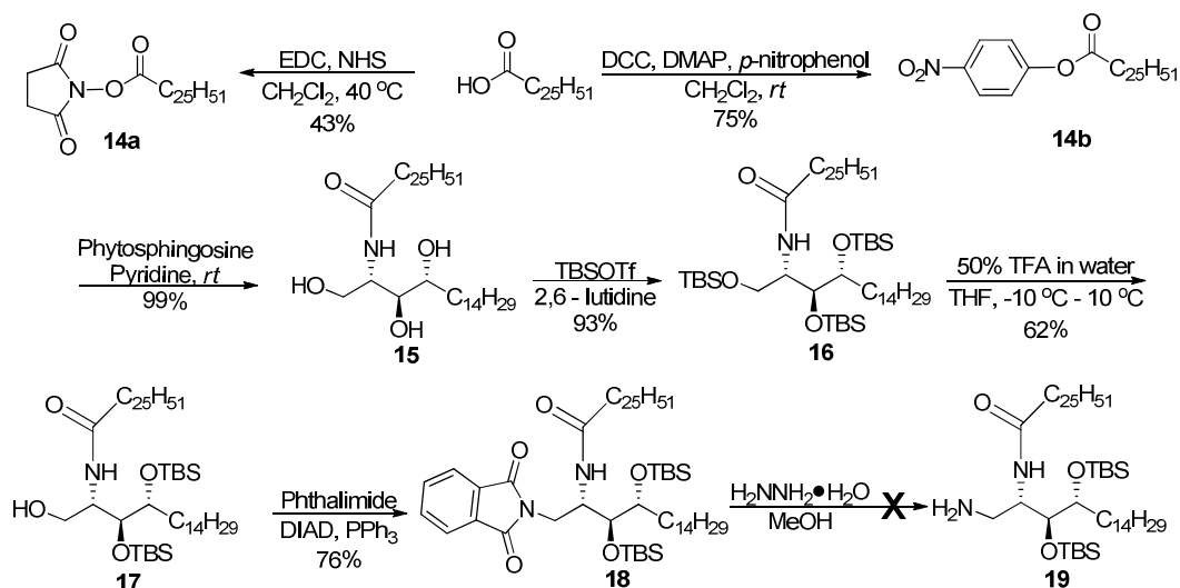
Scheme 6: Attempted synthesis of aminoceramide
