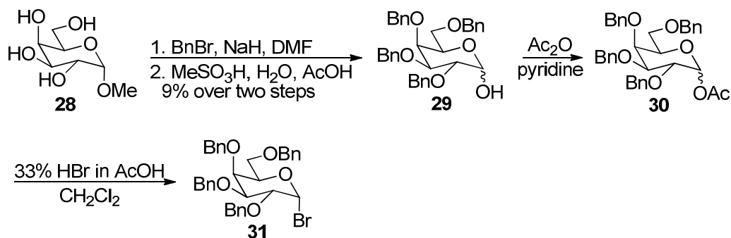
Scheme 8: Synthesis of bromosugar
