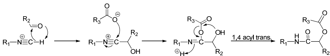
Figure 8: Passerini Reaction.
