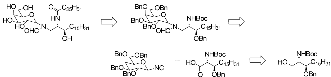
Figure 13: Revised approach to \alpha - N -formyl- N -GalCer
