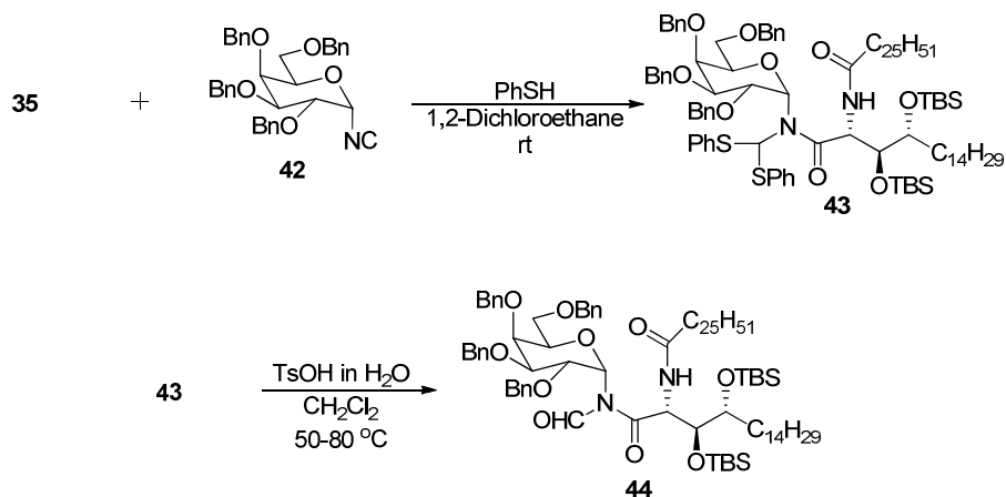
Scheme 13: Formation of N -formyl- N -GalCer using thiophenol
