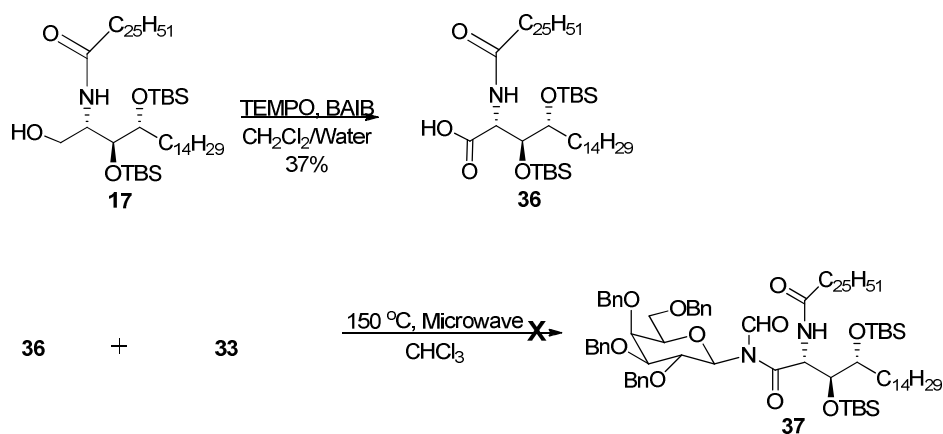
Scheme 11: Attempted synthesis of \alpha - N -formyl- N -GalCer
