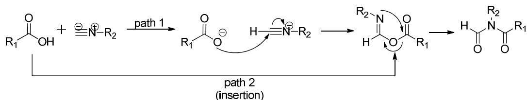
Figure 9: Danishefsky's proposed acyl transformation.
