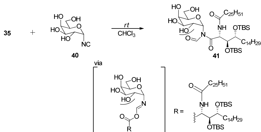
Figure 14: Formation of N -formyl- N -GalCer using unprotected isonitrile
