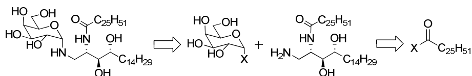
Figure 7: Approach to \alpha - N -GalCer
