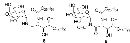
Figure 6: Target \alpha - N -GalCer molecules
