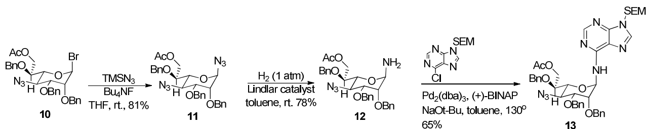
Scheme 4: Formation of alkylglycosylamine using galactose.
