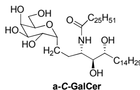
Figure 5: Franck and Tsuji's methylene galactosylceramide 17
