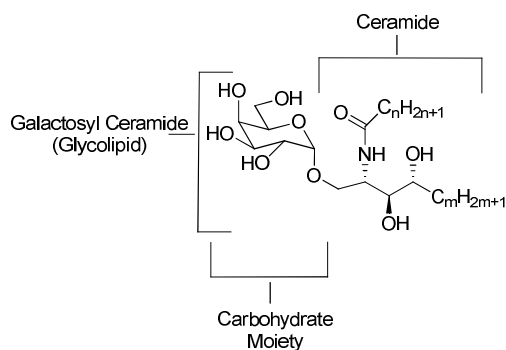
Figure 2: General Structure of Galactosylceramides
