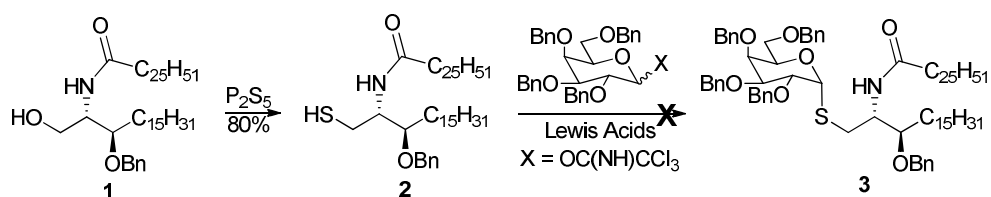
Scheme 1: Glycosylation of a protected \alpha -S-GalCer
