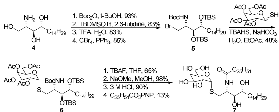
Scheme 2: Synthesis of \alpha -S-GalCer
