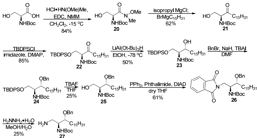
Scheme 7: Synthesis of sphingoid base
