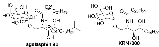
Figure 1: Structures of Agelasphin 9b and KRN7000
