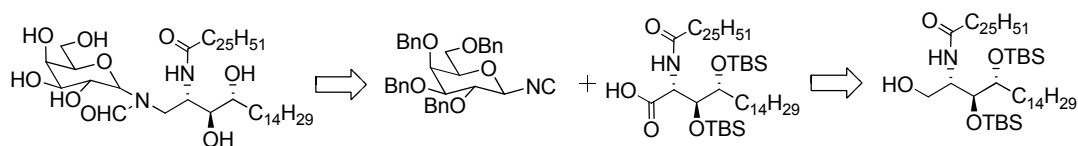
Figure 12: Approach to \alpha -N-formyl-N-GalCer
