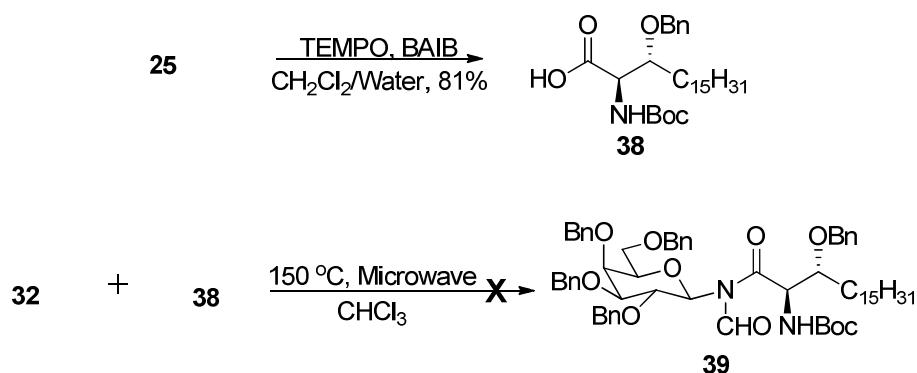
Scheme 12: Attempted synthesis of revised \alpha - N -formyl- N -GalCer
