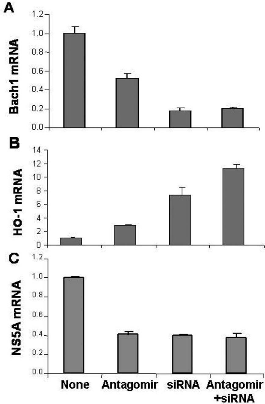
Figure 6. Silencing Bach1 gene up-regulates HO-1 and down-regulates HCV replication in 9–13 cells 9–13 cells were transfected with 50 nM Bach1-siRNA, antagomir of miR-122, or the combination of Bach1-siRNA and antagomir of miR-122 for 48 h, after which cells were harvested. Bach1 (A), HO-1 (B), and NS5A (C) mRNA levels were measured by quantitative RT-PCR, as described in the Methods. Data are presented as means ± SE from three samples.
