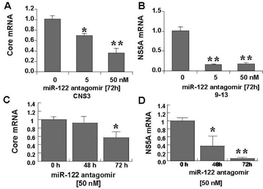
Figure 2. An antagomir of miR-122 reduces HCV RNA abundance in dose- and time-dependent manner in HCV replicon cells Chemically synthesized miR-122 antagomir was introduced into CNS3 and 9–13 replicon cells by Lipofectamine 2000-mediated transfection, and total RNA was extracted 48 or 72 h later. qRT-PCR analysis of HCV core (A) and NS5A (B) mRNAs of cells treated with the indicated dose of miR-122 antagomir for 72 h as shown. Time-courses of replication of HCV core (C) and NS5A (D) treated with 50 nM of miR-122 antagomir are shown. Normalized values of miRNA in absence of miR-122 antagomir were set equal to 1. Data are presented as means ± SE from three samples. * differs from no treatment or zero time, p < 0.05 , ** differs from no treatment or zero time, p < 0.01 .
