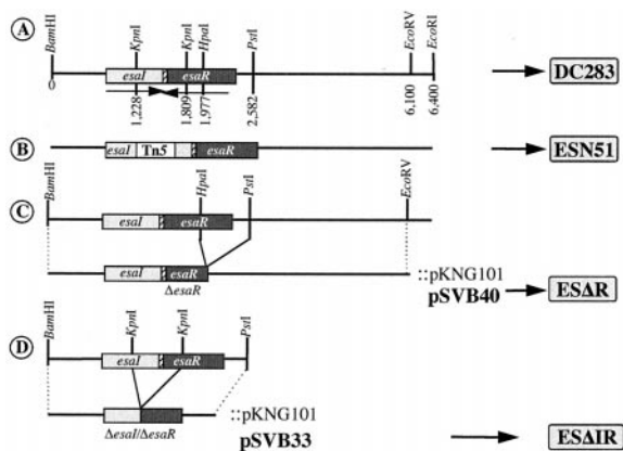
FIG. 1. Restriction map of the esaI/esaR locus (A). The direction of transcription of esaI and esaR is indicated by the arrows. As indicated, a Tn5 insertion in the coding sequence of esaI generates mutant strain ESN51 (B); a HpaI-PstI deletion in the esaR gene is the basis for generating mutant strain ESΔ R (C); a KpnI deletion in esaI/esaR becomes the basis for generating the mutant strain ESΔ IR (D). The stippled region indicates where the coding segments of the two genes overlap.
